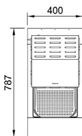
Plan View
