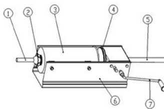
Double speed Rack sausage stuffer/filler Horizontal
