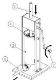
Single speed Threaded Rod sausage stuffer/filler vertical
