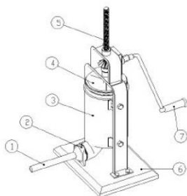
Single speed Threaded Rod sausage stuffer/filler vertical
